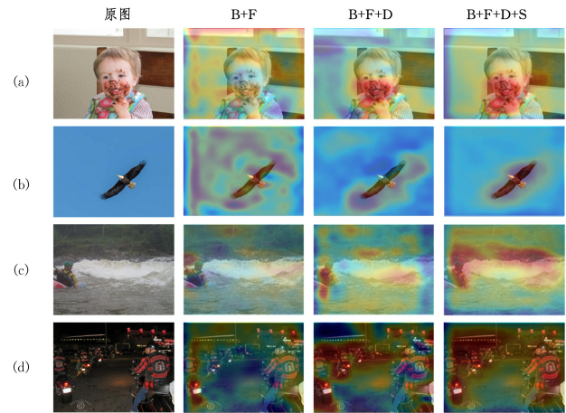
图 8 在 baseline 的基础上引入各模块的情感注意力图 Fig. 8 Sentiment attention map after each module is introduced based on baseline
